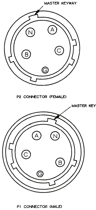
Figure 6. 40/60-amp, 5-wire Connector Face/ Key Positioning.
