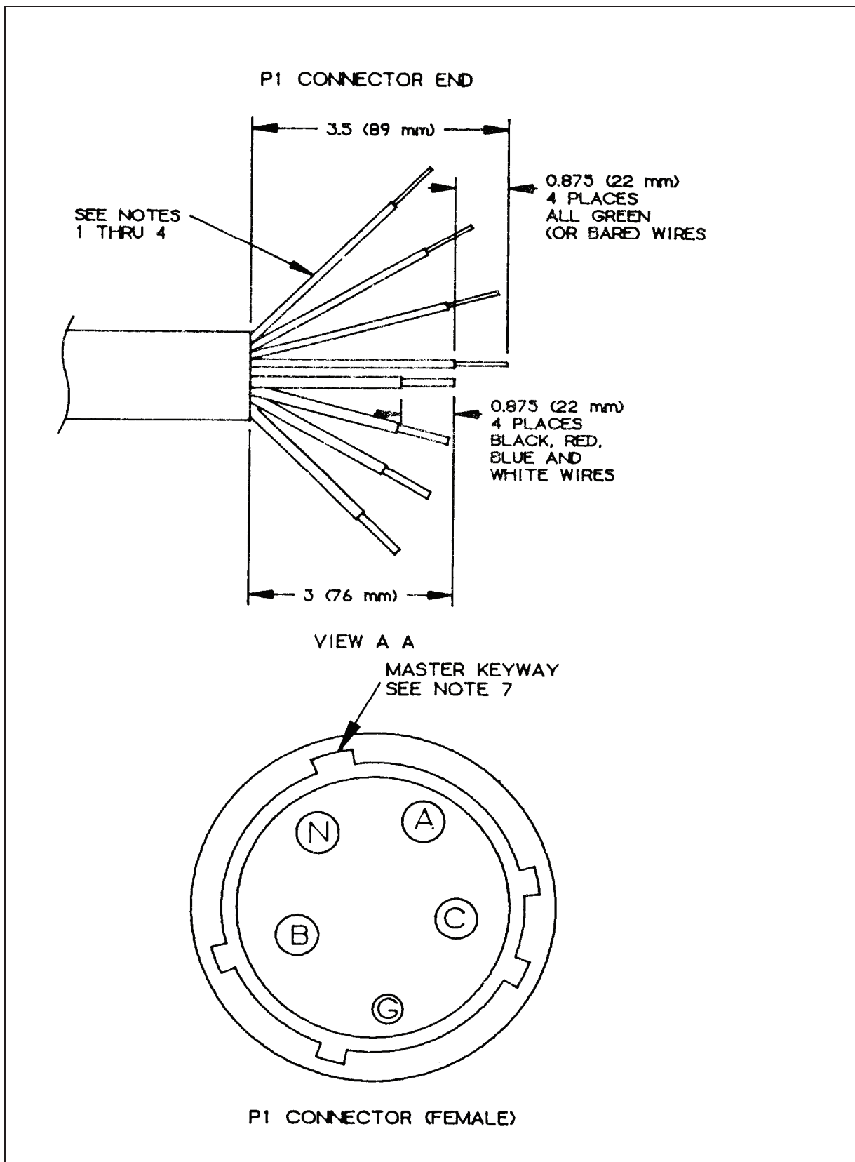
Figure F-17. Pigtail Cable, 40/60-Amp, (4-ft). (2 of 2)
