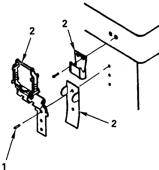
Figure 1. Latch Assembly
