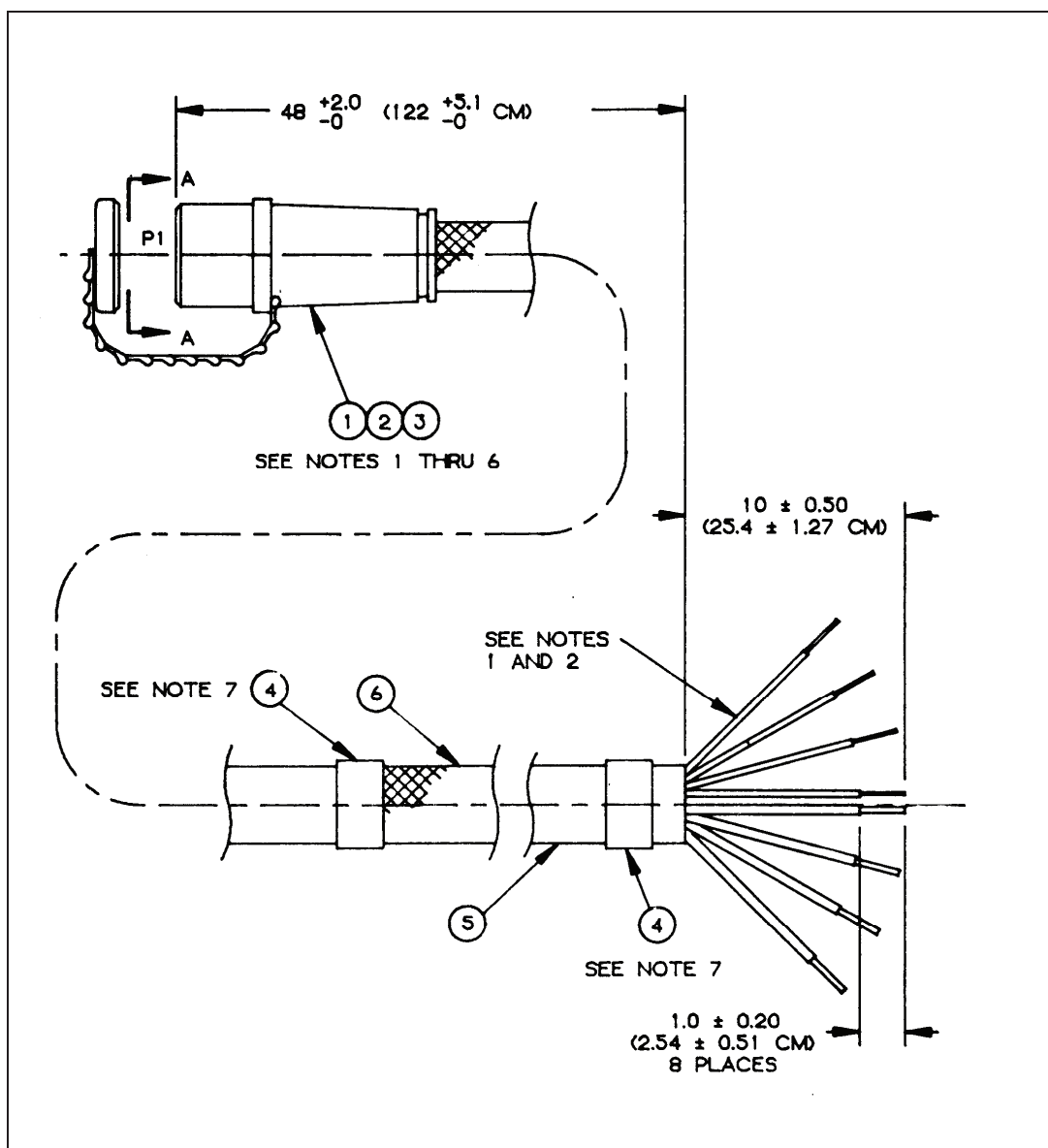
Figure F-15. Pigtail Cable, 200-Amp, (4-ft). (1 of 2)
