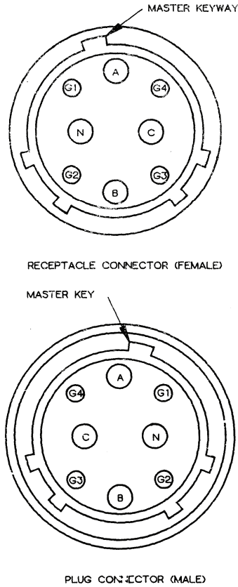
Figure 5. 200 and 100-amp, 8-wire Connector Face/ Key Positioning
