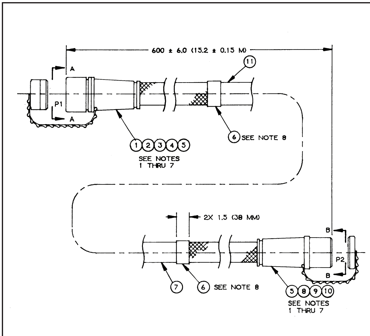
Figure F-21. Service/Feeder Cable, 200-Amp, 40/60-Amp (25-ft). (1 of 2)
