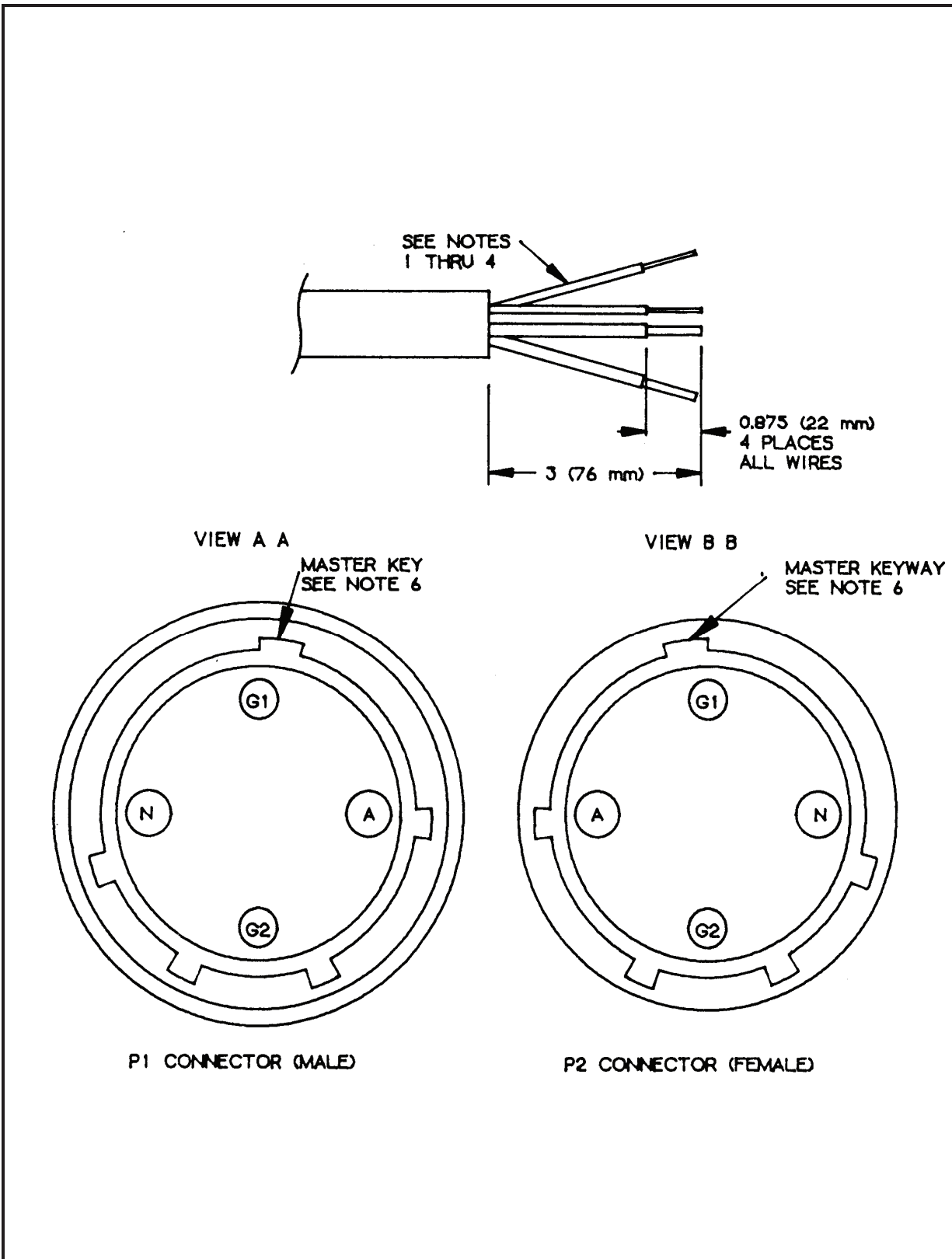
Figure F-3. Service/Feeder Cable Assembly, 60-Amp, (50 ft) (2 of 2)
