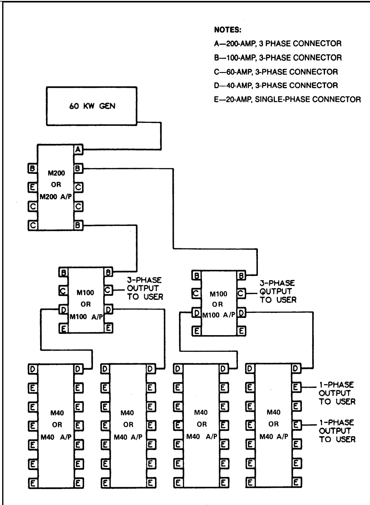
Figure 8. Example of Network Arrangement.
