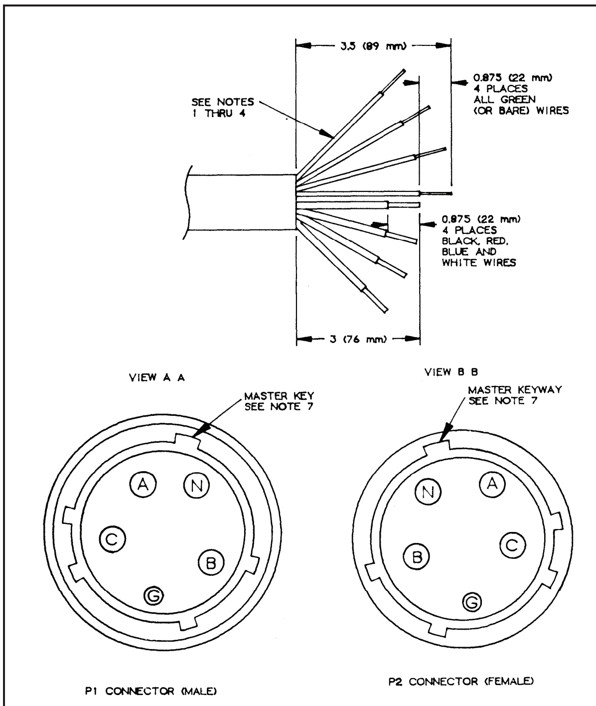
Figure F-21. Service/Feeder Cable, 200-Amp, 40/60-Amp (25-ft). (2 of 2)
