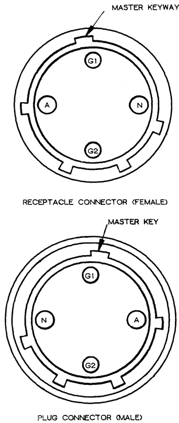
Figure 8. 20-amp, 3-wire Connector Face/ Key Positioning.
