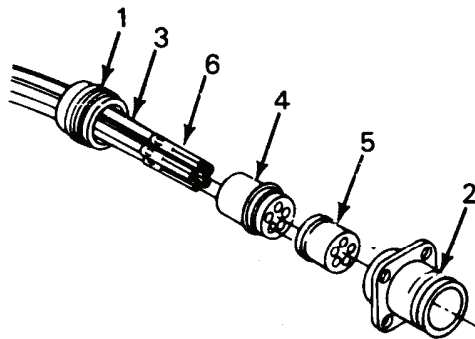
Figure 1. Connector Layout
