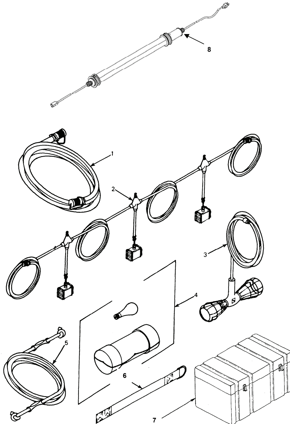
Figure 7. Electrical Utility Kit Assembly, M46.
