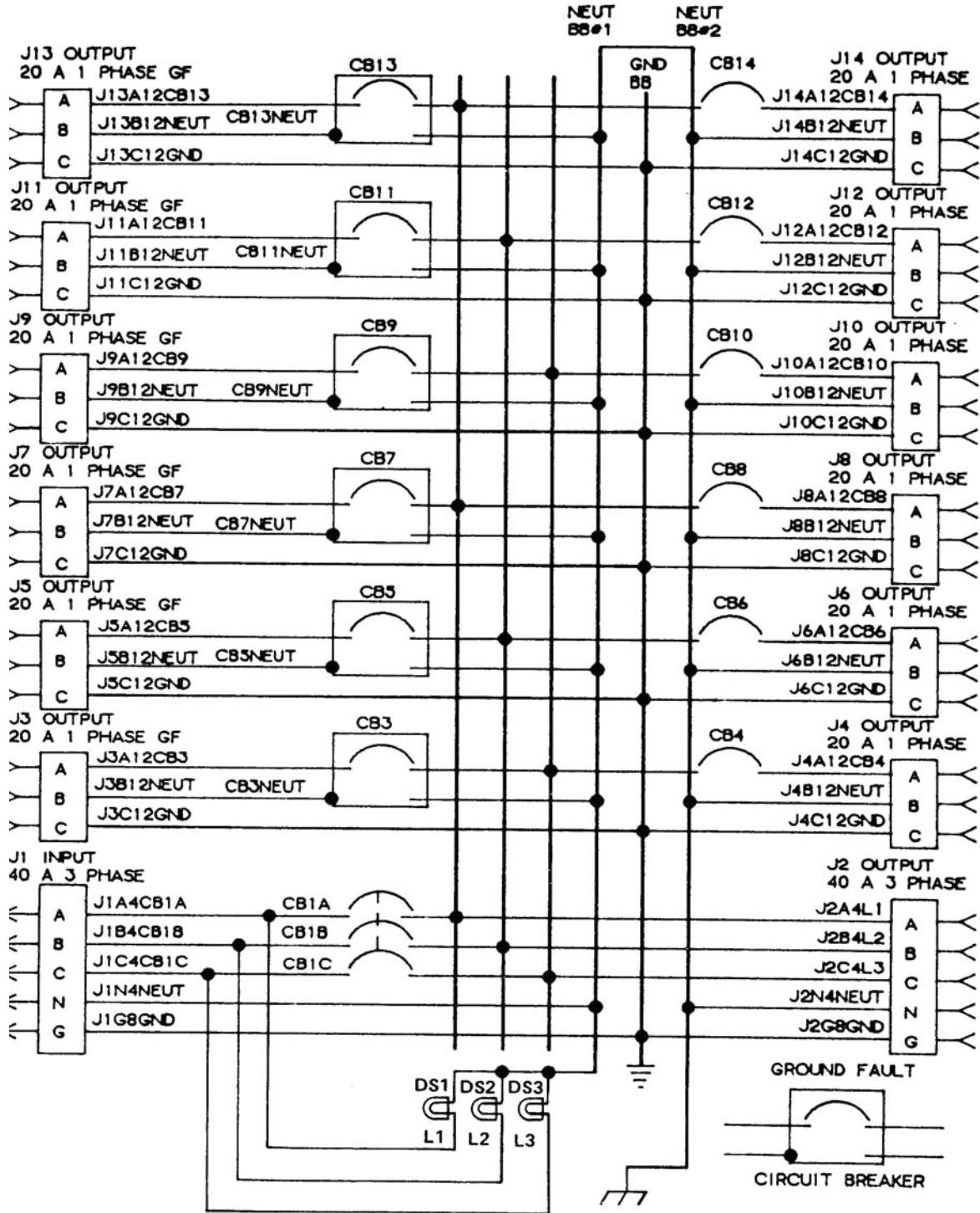
Figure 3. M40 (DISE) Distribution Center Wiring Diagram.
